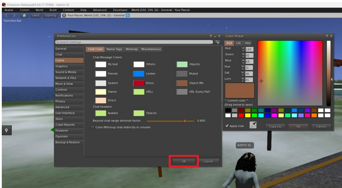
Figure 19: Select Color
